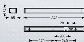
Acuro S 114...04
