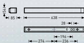
Acuro S 114...01
