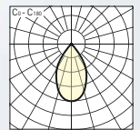
AthenikL C05 MR-CAT2 LED 2000 nw... UTE: 0.94 A + 0.00 T DIN 5040: A70 CIBSE: BZ 1 NBN L 14-002: BZ 1
