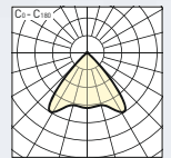
AthenikL C05 MR LED 2000 nw... UTE: 0.94 A + 0.00 T DIN 5040: A60 CIBSE: BZ 1 NBN L 14-002: BZ 1
